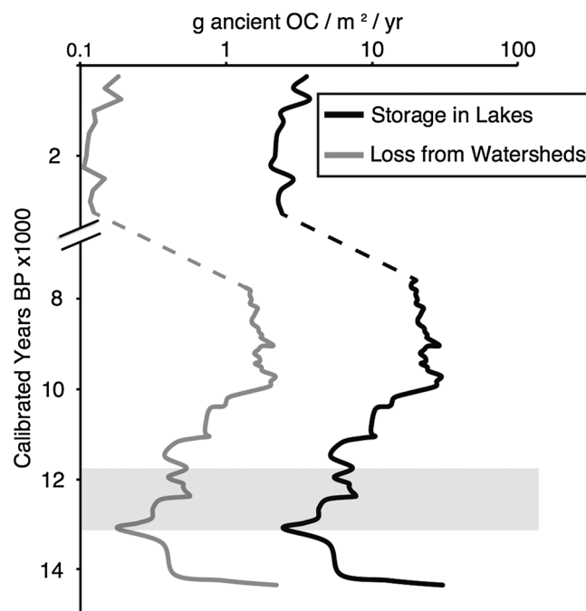
Figure 11. Estimated rates of ancient OC ( >1.0 ka OC) deposited in LOP (14.4–7.7 ka) and Nikivlik Lake (3.3 ka–present) on a per year basis (black line). Estimated rates of the loss of ancient OC from the lakes' watersheds (gray line). The dashed line represents the interpolated pattern that occurs during the gap between the LOP and Nikivlik Lake records. Gray shading represents the Younger Dryas chronozone.
