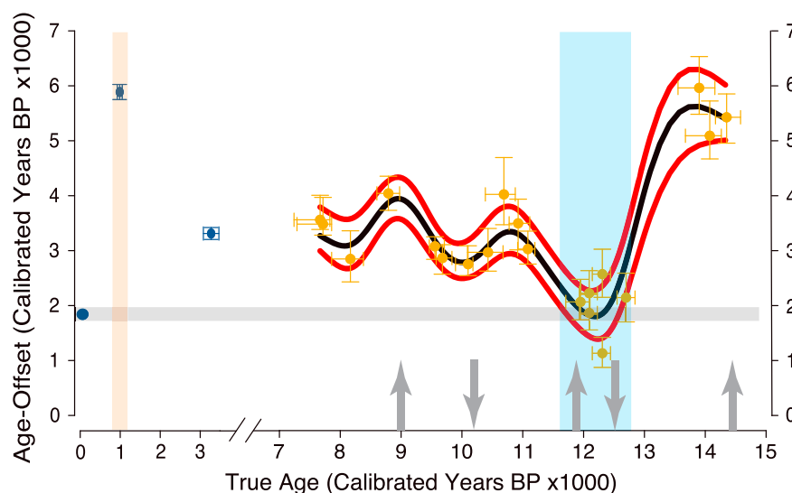
Figure 6. Summary of ^{14}\text{C} age-offsets in Nikivlik Lake (blue points) and in the LOP section (gold points). Points represent median values of calibrated ^{14}\text{C} age-offsets, and bars show the 2\sigma ranges of age-offsets (LOP; n = 20 dates, Nikivlik Lake; n = 3 dates). Black and red lines are the mean and 95% upper and lower limits of the interpolated age-offset cubic spline model constructed from the bulk ^{14}\text{C} dates. Horizontal gray shading is the 95% range of the age-offset observed from the surface sediments of Nikivlik Lake. Blue shading denotes the Younger Dryas chronozone. The three data points to the left are from Nikivlik Lake, the modern lake that still occupies the LOP basin. Orange shading denotes the Medieval Warm Period chronozone. Gray arrows are periods of lake-level deepening (up) and lowering (down) as inferred by sedimentology.
