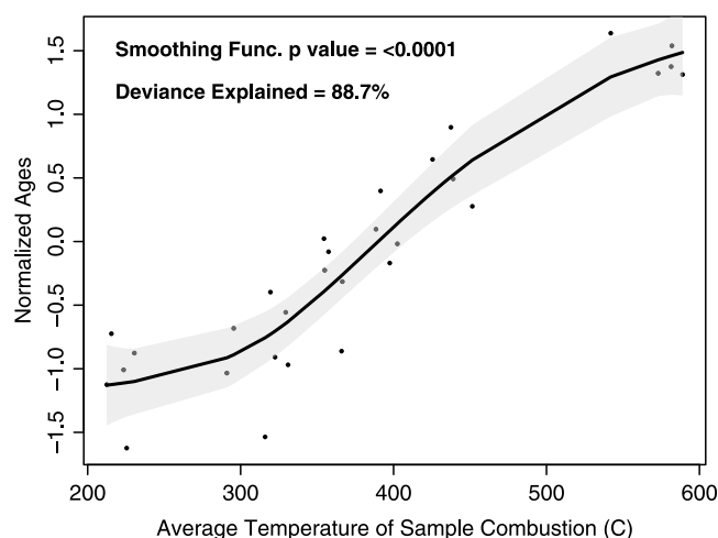
Figure 10. Normalized ^{14}\text{C} ages of ramped-temperature gas samples. Black line and gray shading are the mean and 95% confidence intervals for a general additive model fitted to the data. OC that is more resistant to decay has the highest ^{14}\text{C} age and is evolved from the sediment sample at the highest temperatures.
