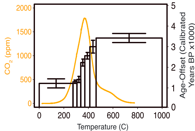
Figure 7. An example of thermogram and ^{14}\text{C} age-offsets of ramped-temperature ^{14}\text{C} analysis. Data are from Unit 4 in the LOP section. The \text{CO}_2 curve is the gas concentrations evolved at successively higher temperatures, and the age-offset shows the ^{14}\text{C} age-offset of the gas collected at each temperature step. The age-offset axis is zeroed to the true age for this sediment layer (11.1 ka).
