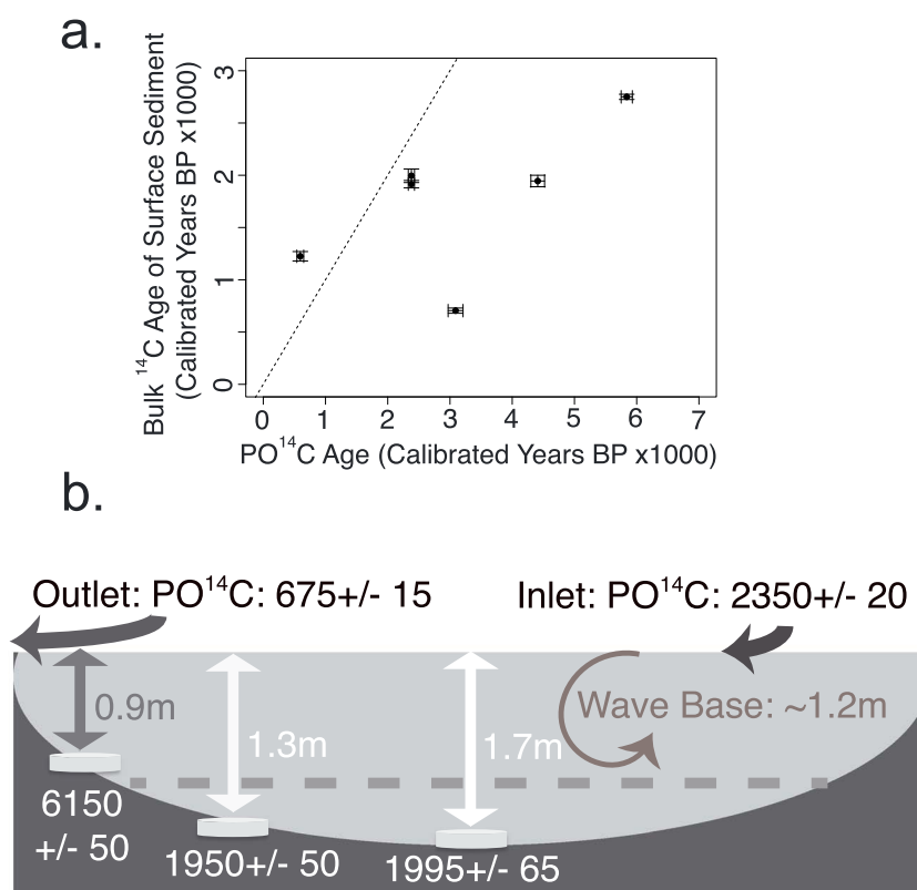
Figure 3. (a) Scatterplot showing particulate organic carbon radiocarbon age ( \text{PO}^{14}\text{C} ) of inlet water and age of surface sediments in LOP watershed lakes excluding the nearshore deposit in Nikivlik Lake (the core sampled from 0.9 m water depth). The dotted line represents the 1:1 relationship and illustrates that all but one lake has older OC entering through the inlet than is being deposited in the sediment. (b) \text{PO}^{14}\text{C} ages of surface sediment samples and entering and exiting Nikivlik Lake.
