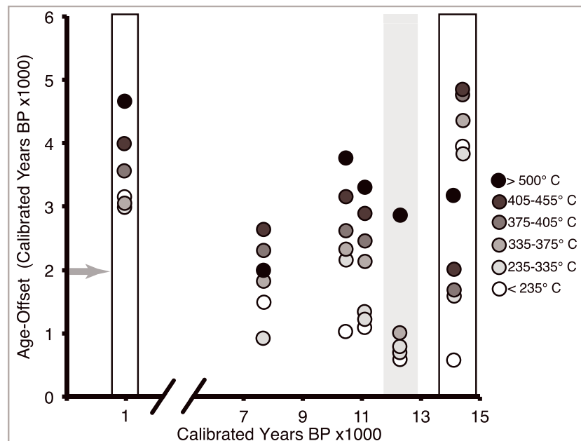
Figure 8. Ramped-temperature ^{14}\text{C} age-offsets of individual gas samples and the average temperature range the gas samples were heated. Episodes of inferred thermokarst-driven mass movements are represented by black boxes. Black box on the right is the Bølling-Allerød chronozone while the left black box corresponds to the Medieval Warm Period chronozone. The Younger Dryas chronozone represented in gray shading. Gray arrow is the current age-offset for Nikivlik Lake.
