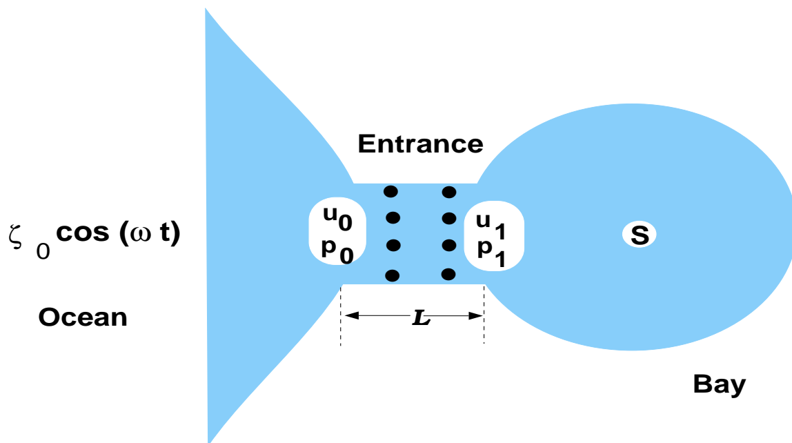
Figure IV.20. Schematic representation of tidal power construction and hydrodynamical modeling in the bay. At the ocean side the tide is prescribed as \zeta_0 \cos(\omega t) , dots depict the tidal current generators located in the entrance to the bay.
