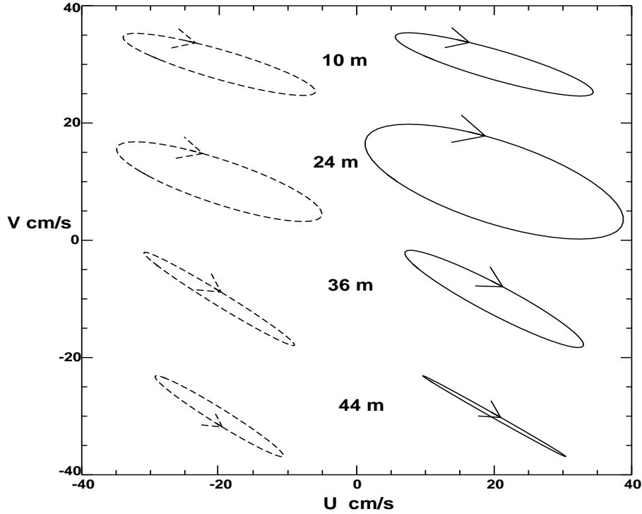
Figure III.17. M_2 tidal ellipses at the mooring F8 during summer period. Calculations are given by broken lines, observations by continuous lines. Depth is shown as distance from the free surface.
