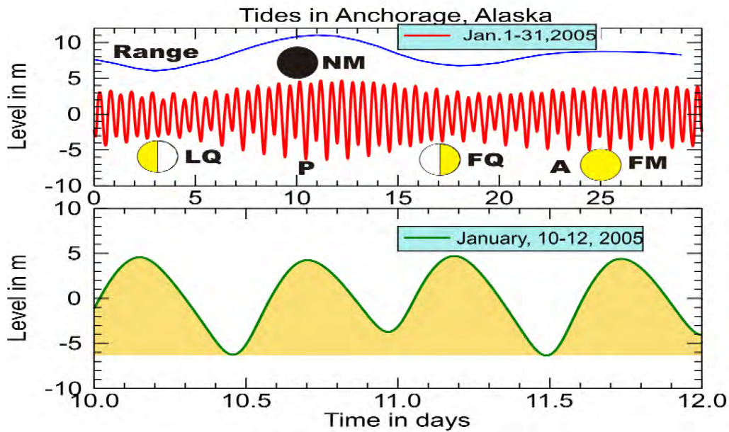
Figure V.6 Monthly series of the sea level data, January, 2005, Anchorage, Alaska (upper panel) and two-day series (lower panel). Moon phase are: FM-fool moon, NM- new moon, FQ-first quarter, LQ- last quarter. P and A denote Moon’s perigee and apogee. Blue line: tidal range.
