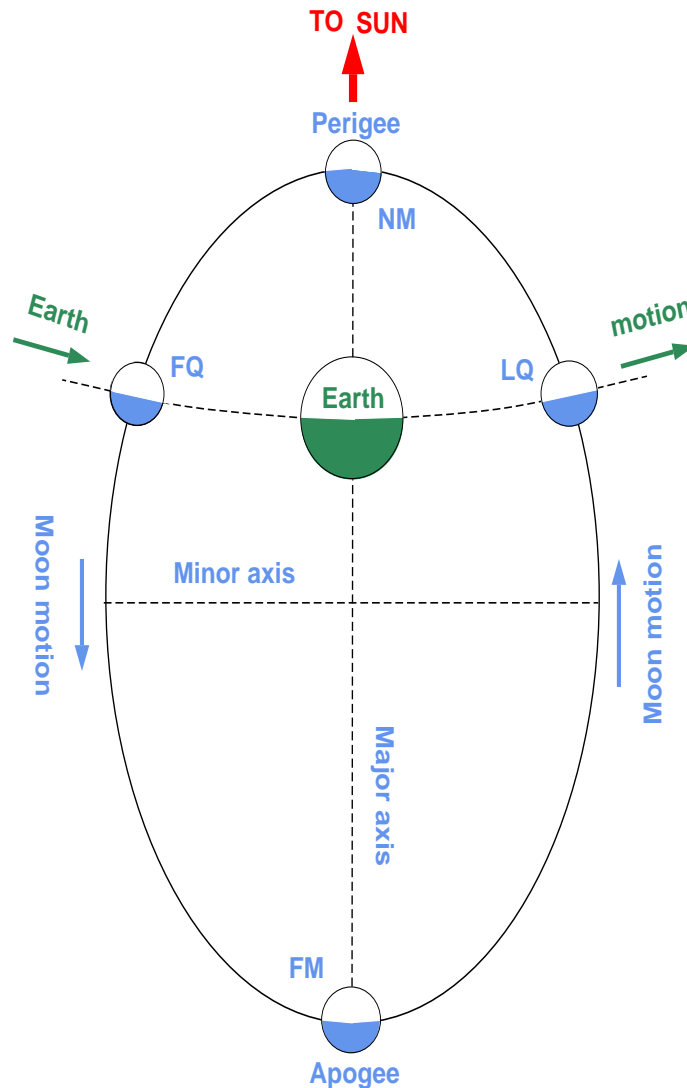
Earth, Moon and Sun at Syzygy
