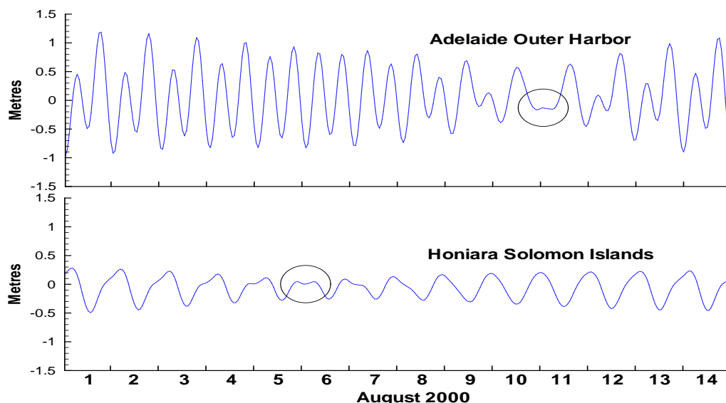
Figure VI.3 Sea levels at Adelaide and Honiara. Intervals with virtually no tidal variation are encircled. In Adelaide these intervals are called the "Dodger Tide".
