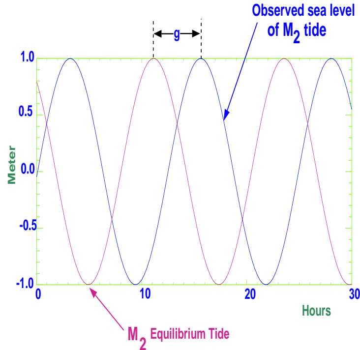
Figure V.9 Phase lag g of the M_2 tidal constituent
