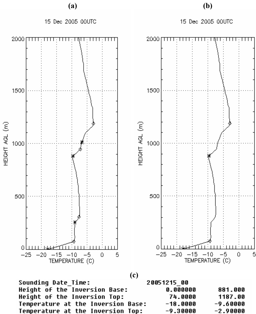
Figure 2.6 Inversion layers detected by the algorithm. (a) Temperature profile showing the four inversion layers initially detected by the algorithm. The * represents the base and the ◇ represents the top of the of the inversion layers (b) Final two inversion layers selected by algorithm (c) Altitude and temperature data for the two inversion layers shown in Fig. 2.6b.
