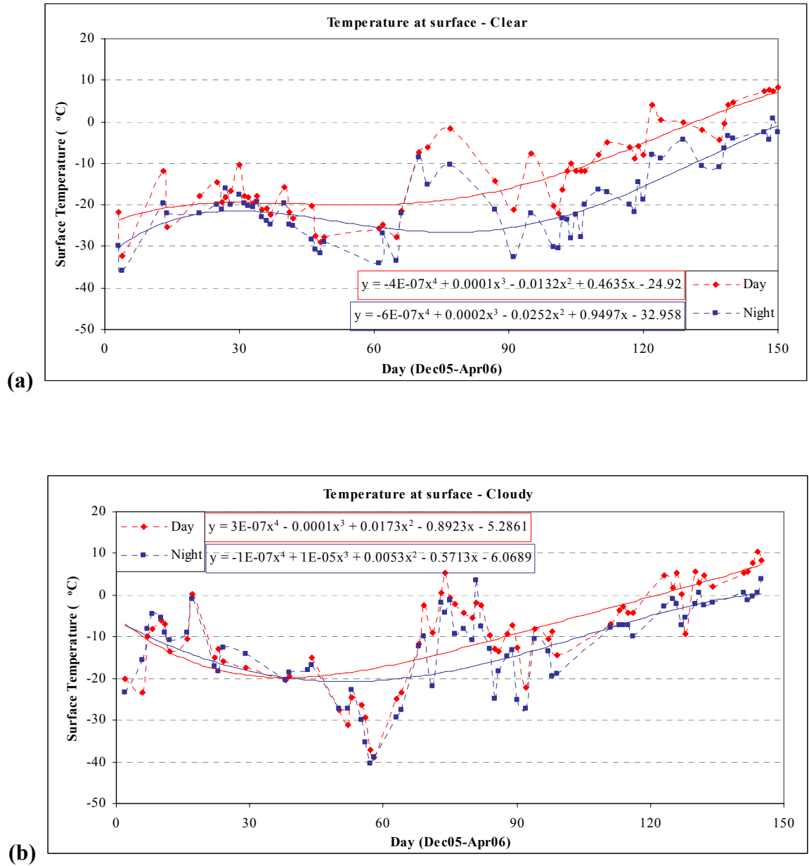
Figure 3.6 Surface temperatures for clear and cloudy conditions. (a) The surface temperatures for the chosen clear nights are shown in blue and the corresponding daytime temperatures for those clear nights are shown in red. (b) Surface temperatures for the chosen cloudy nights are shown in blue and the corresponding daytime temperature for those cloudy nights are shown in red.
