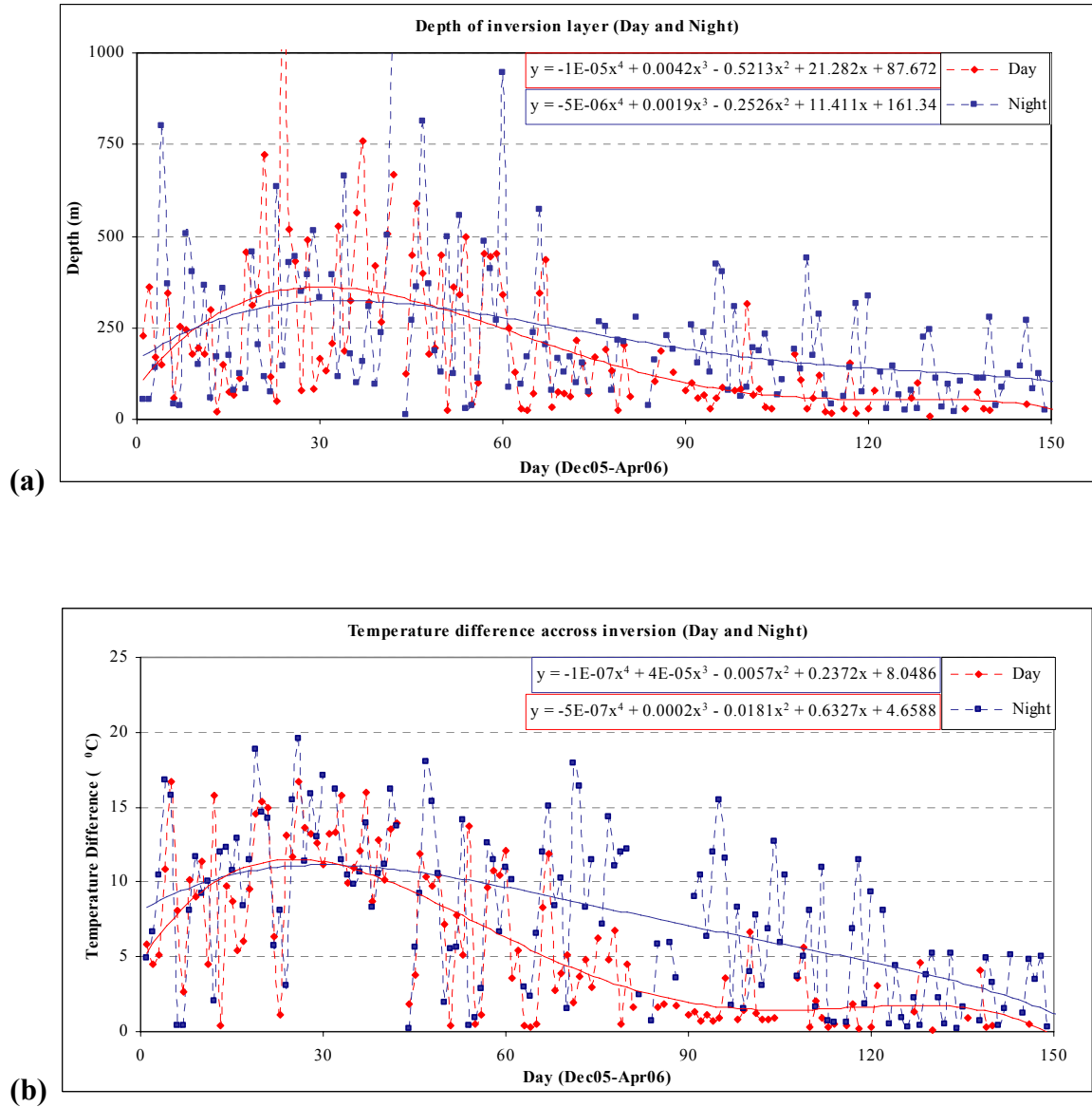
Figure 3.4 Characteristics of the inversion layer for day and night. Characteristics of the lowest inversion layer shown in Figure 3.2 plotted separately for day and night. (a) Depth of the inversion layer and (b) temperature difference across the inversion layer.
