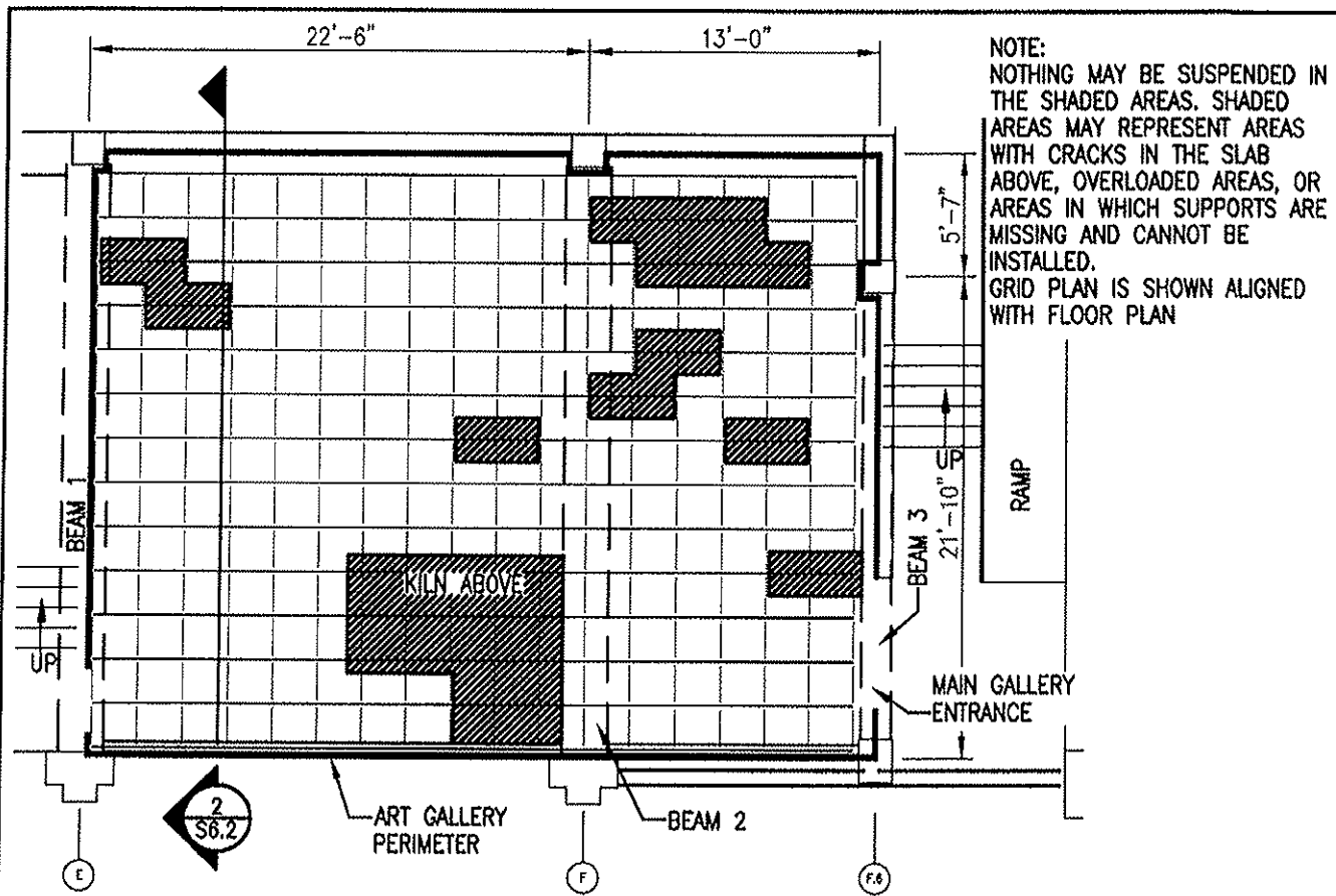
1 GRID PLAN S6.2 NO SCALE
