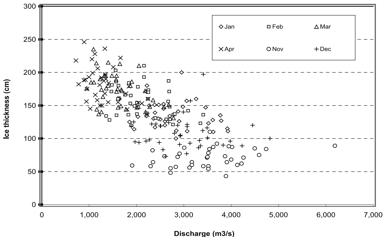
Figure 6. Relationship between stream flow and river ice thickness at the Kusur station during November to April.
