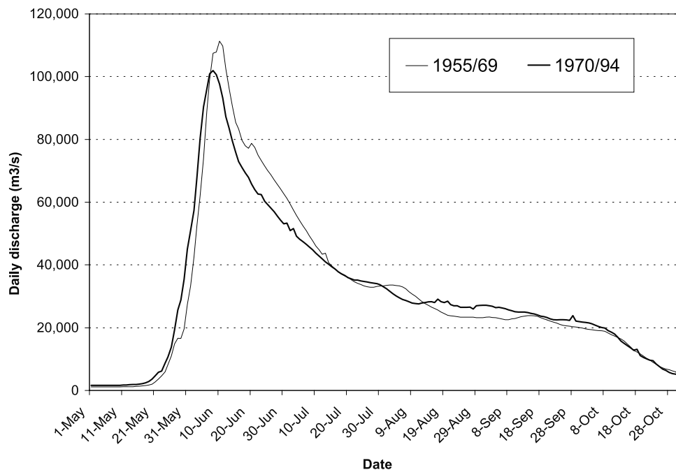
Figure 4. Comparison of long-term mean daily stream flow regimes at Kusur station, 1955–1969 versus 1970–1994.
