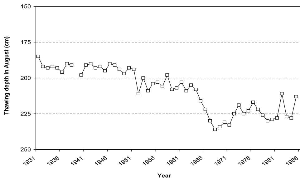
Figure 11. Thaw depth of the active layer at the end of August in Yakutsk, 1931–1985.
