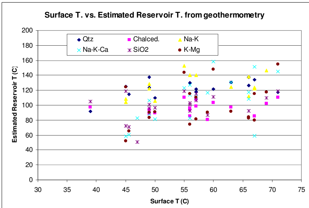
Figure 2.7. Natural surface temperatures vs. estimated reservoir temperatures for CAHSB fluids. Estimated reservoir temperatures calculated from six different geothermometry methods: Quartz, Chalcedony, Na-K, and Mg-corrected Na-K-Ca geothermometers (Fournier, 1981) plus SiO 2 and Mg-K geothermometers from Giggenbach (1988).
