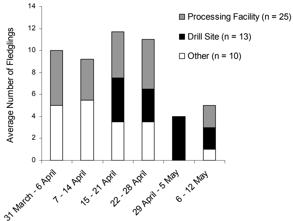
Figure 3.7. Average number of fledglings produced relative to nest initiation dates for each type of structure ravens used for nesting in Alaska's North Slope oil fields. Other includes inactive drill rigs, ARS (U.S. Air Force Alaska Radar System) towers, and bridges.
